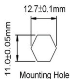
Mounting Hole
